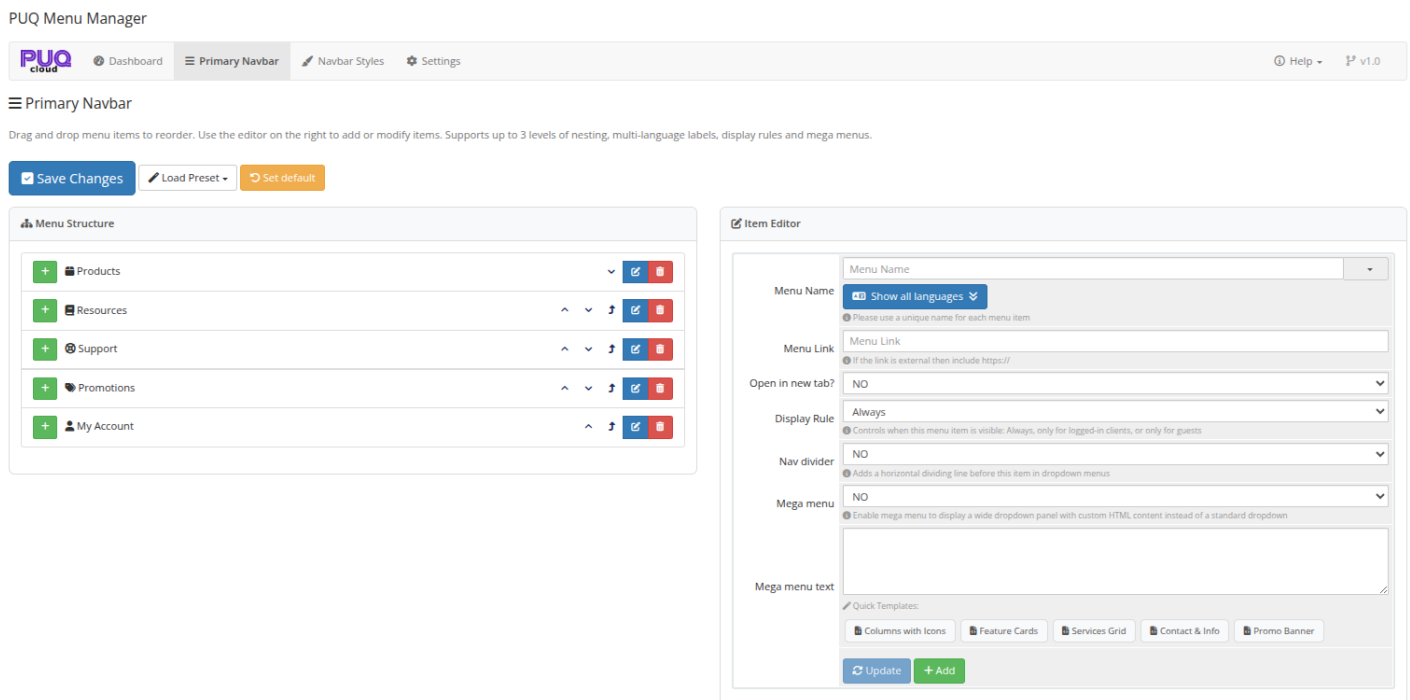
Primary Navbar editor — drag-and-drop menu structure on the left, item editor on the right
